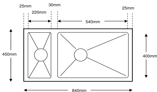
Elkay EC-22128 (Reversible Double Bowl) Size: 840x450x230mm
