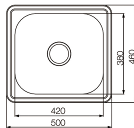
Elkay ECLH-212 (Single Bowl) Size: 500x460x200mm
